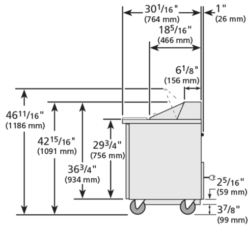
RIGHT VIEW
