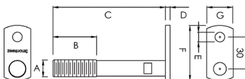
304 Grade Stainless Steel Adjustable Lug Foot
