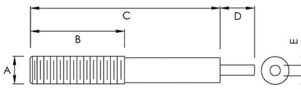
304 Grade Stainless Steel Adjustable Pin Foot
