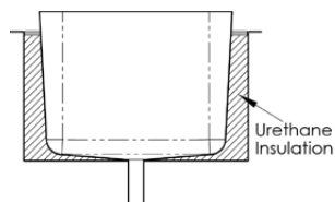
Cross Section
