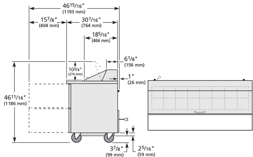
RIGHT VIEW
