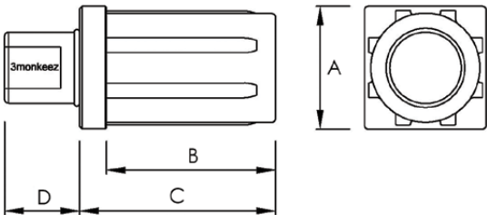
Nylon Adjustable Foot - Square Tube
