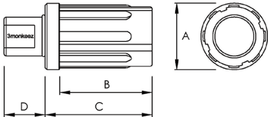
Nylon Adjustable Foot - Round Tube
