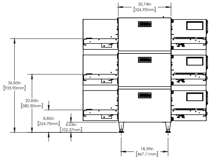
PS2020 Front View Triple Stacked Units
