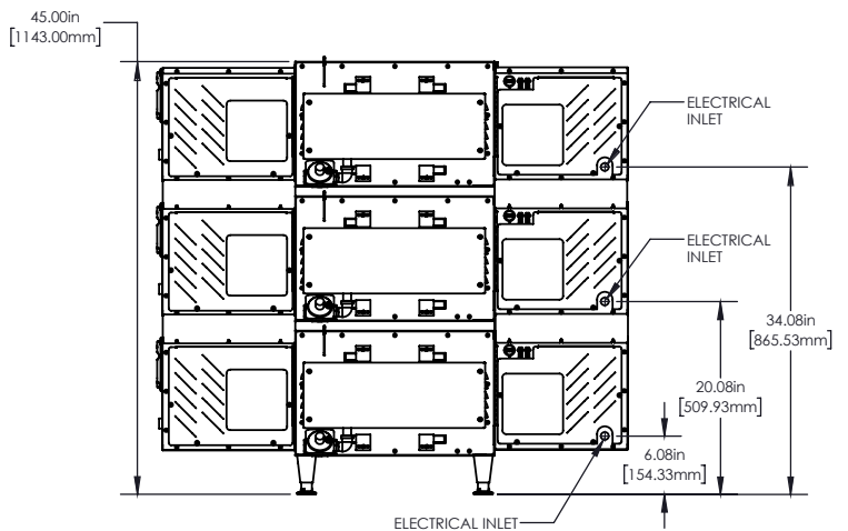
PS2020 Rear View Triple Stacked Units
