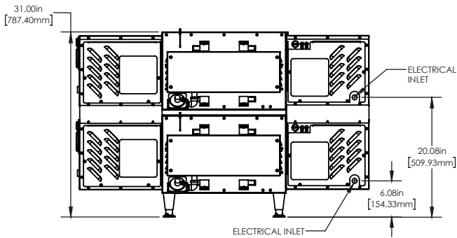
PS2020 Rear View Double Stacked Units
