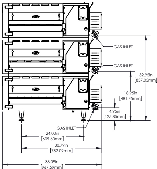
PS2020 Side View Triple Stacked Units
