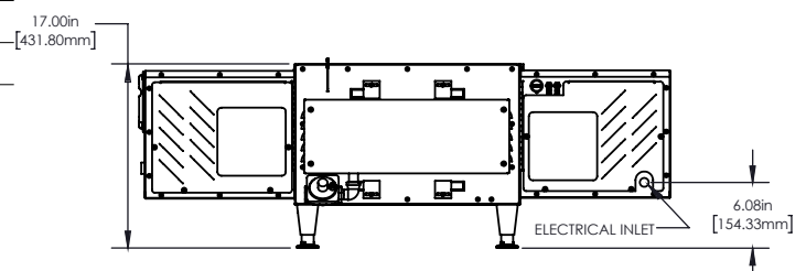
PS2020 Rear View
