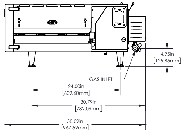
PS2020 Side View
