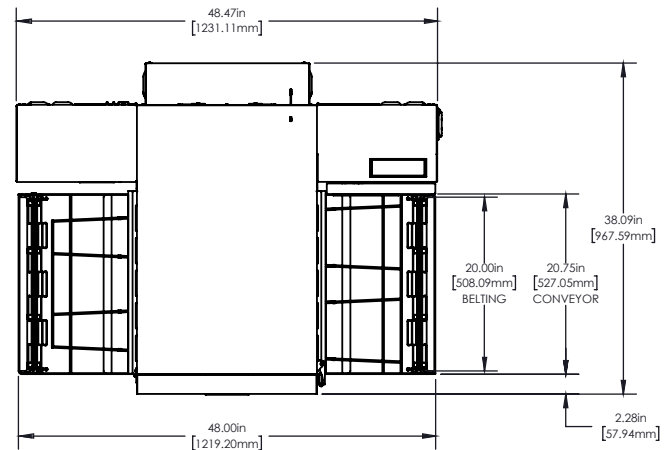
PS2020 Top View
