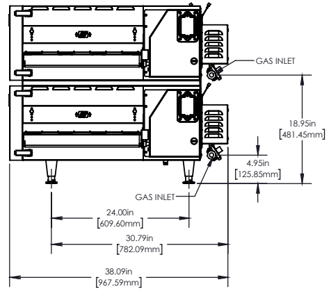
PS2020 Side View Double Stacked Units
