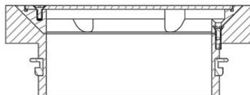
Cross Section
